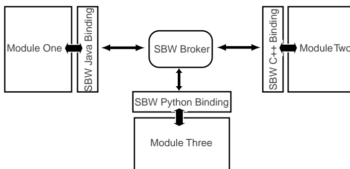
FIG. 1. Connection between broker, modules, and binding libraries.
