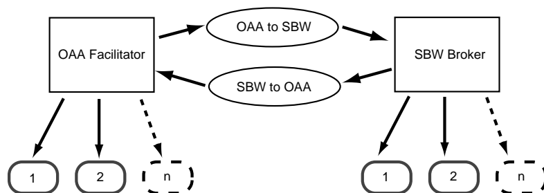
FIG. 9. Structure of the BioSPICE/SBW bridge.
