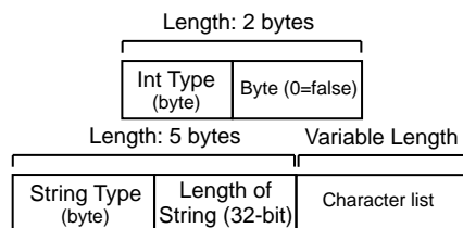
FIG. 6. Boolean and string data types.
